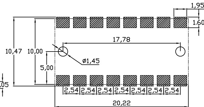
RECOMMENDED PCB LAYOUT TOP VIEW (. XX \pm 0. 05)
